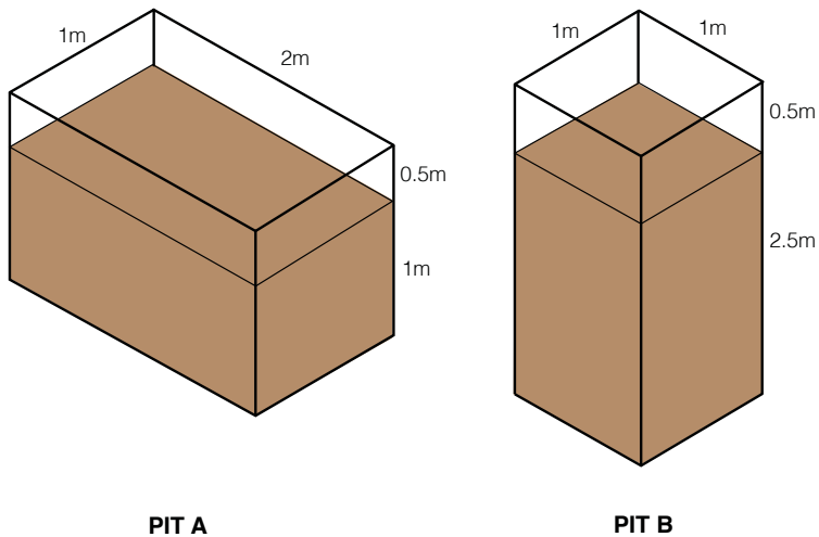
Figure 6. Two pits with the same total volume but a different effective volume
