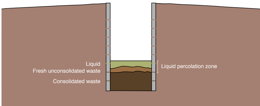
Figure 6. Liquid percolation zone in a pit latrine
