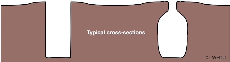
Figure 5. Typical pit latrine shapes
