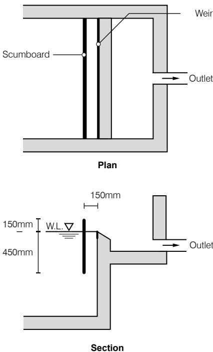
Figure 9. Tank outlet using overflow weir
