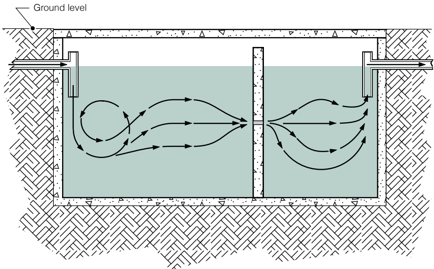
Large tank – turbulence takes up a much smaller proportion of the first tank
