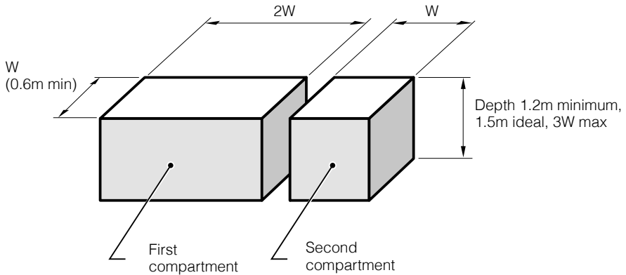
Figure 7. Tank dimensions for liquid, scum and sludge volume
