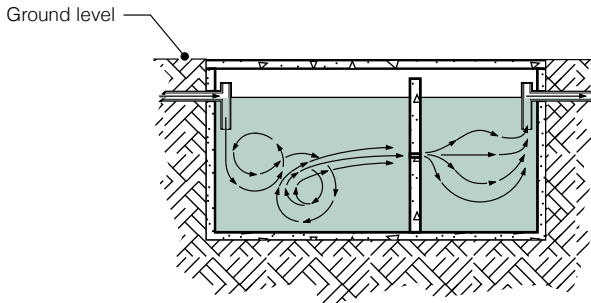
Small tank – turbulence takes up a large proportion of the first tank
