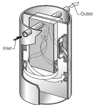
Figure 11. Examples of pre-fabricated septic tanks
