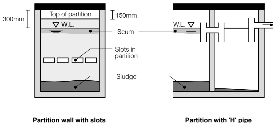
Figure 10. Options for flow through tank partitions
