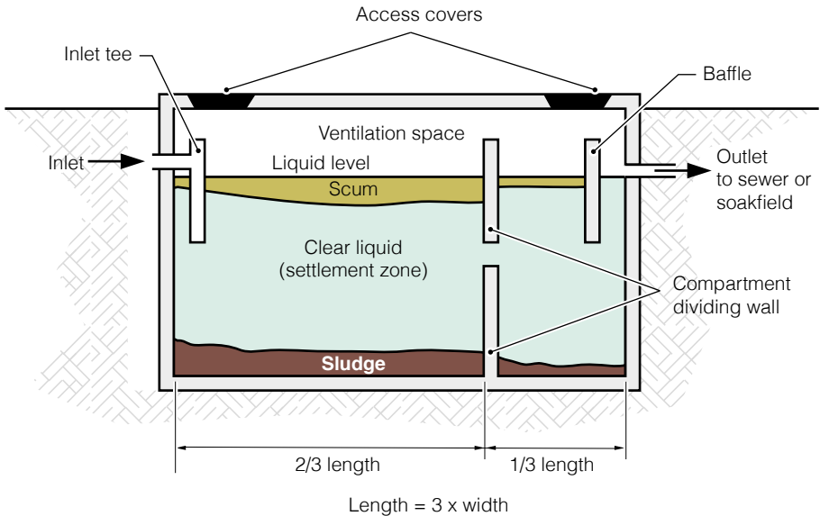
Figure 5. Treatment process in a septic tank
