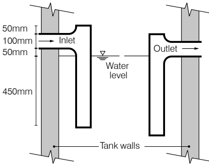
Figure 8. Tank inlet and outlet pipes
