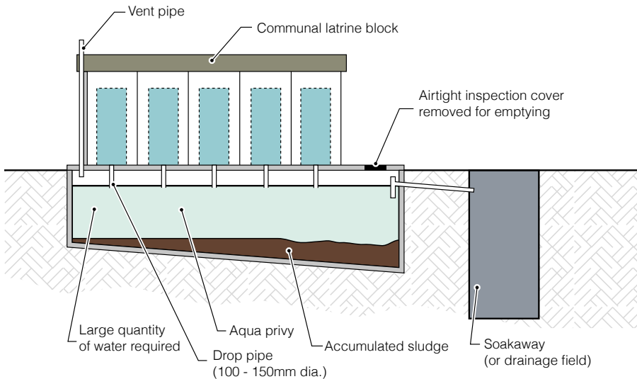
Figure 4. An aqua-privy for a communal latrine (e.g. a school)
