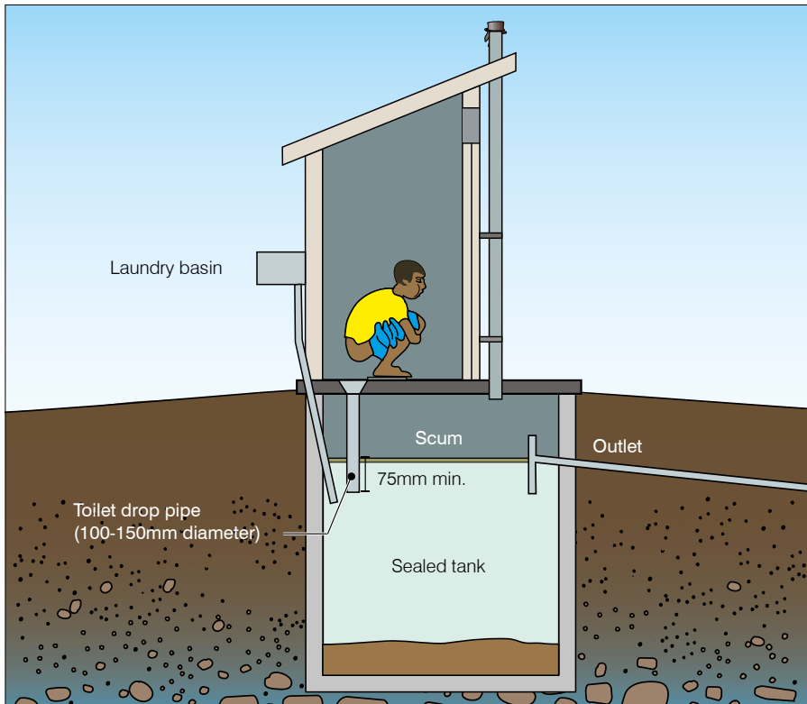
Figure 3. An aqua privy
