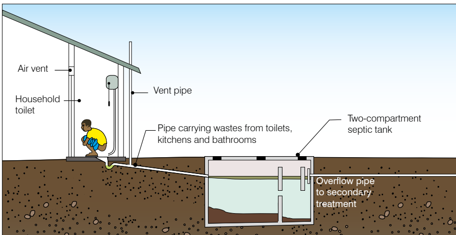
Figure 1. Wastewater treatment using a septic tank
