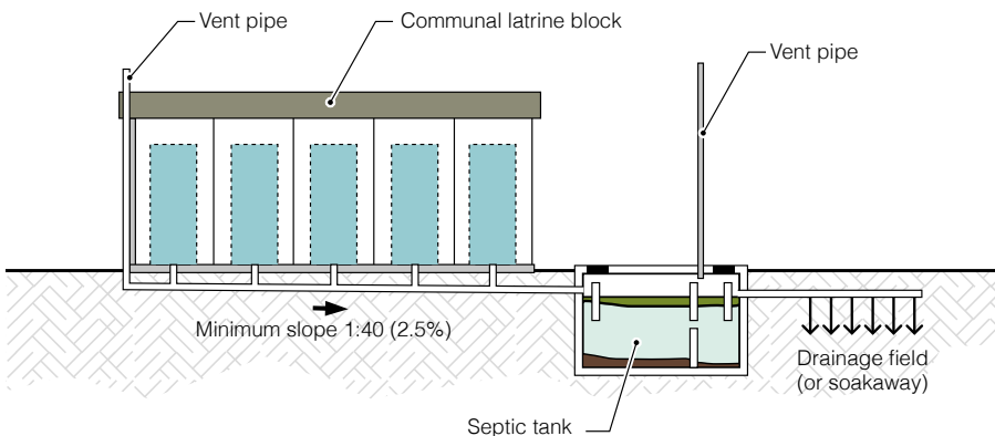
Figure 2. Communal toilet connected to a septic tank and drainage field
