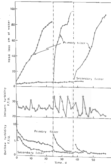
Fig. 4 Series filtration using rice hull ash medium.
