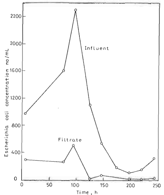
Fig. 3 Bacterial removal by rice hull ash medium depth = 750mm ; porosity = 93.5% rate of filtration = 1.0 \text{ m}^3/\text{m}^2 \text{ h}
