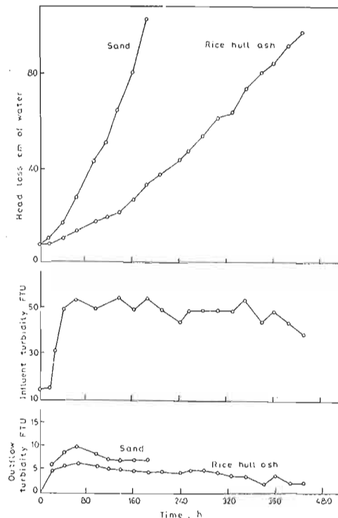
Fig. 1 Performances of sand and rice hull ash media at 1 \text{ m}^3/\text{m}^2 \text{ h} Depth of medium = 750 mm
