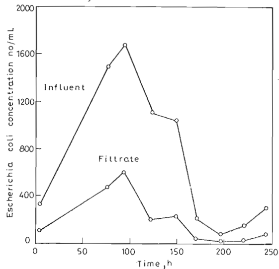
Fig. 2 Bacterial removal by sand medium rate of filtration = 1.0 \text{ m}^3/\text{m}^2 \text{ h} depth = 750 mm; porosity = 44%
