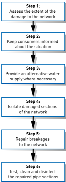
Figure 1. Steps for rehabilitating a small-scale piped water distribution system
