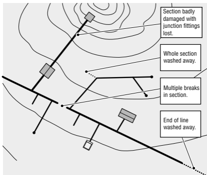
Figure 2. Map of a piped distribution network with a record of damage
