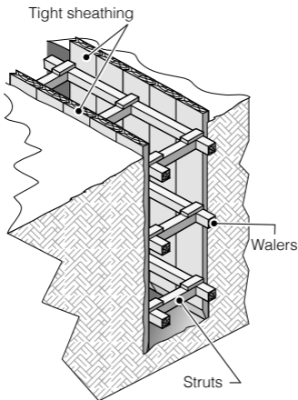
Figure 6. Shoring the work area
