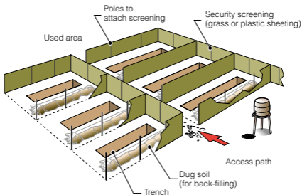
Figure 4. Trench defecation fields
