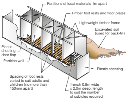
Figure 5. Deep trench latrines
