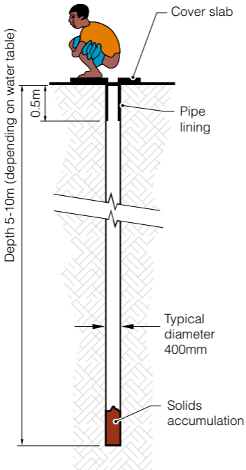
Figure 7. A borehole latrine
