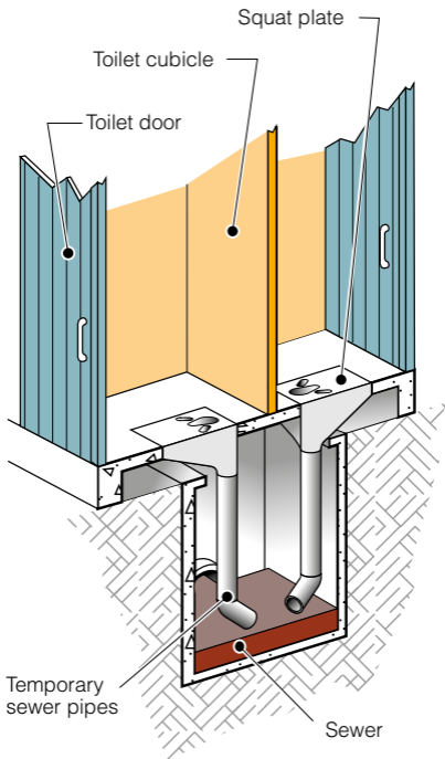
Figure 6. Temporary toilet over a sewer
