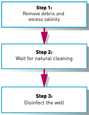
Figure 1. Steps for cleaning a saltwater-contaminated well
